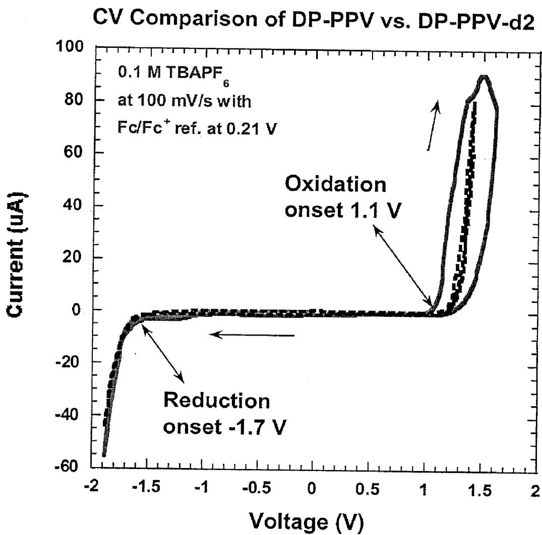
Figure 2. Cyclic voltammetric curve of normal DP-PPV (dotted line in blue) and duterated DP-PPV-d2 (solid line).
